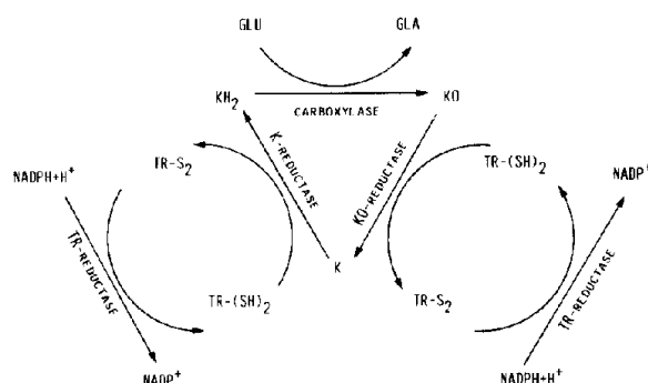
Fig.3. Proposed extension of the vitamin K cycle. The synthetic dithiols from fig.1 have been replaced by thioredoxin-(SH) 2 and the thioredoxin-(SH) 2 generating system (thioredoxin reductase + NADPH). TR, thioredoxin.
